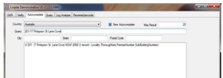
2017Q1.0 Correct output when input has slash
